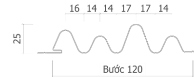
W-30 panel
