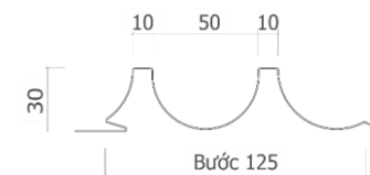
D-50 panel
