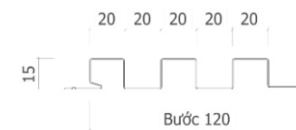
F-20 panel
