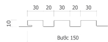
F-30 panel
