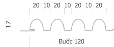
W-20 panel
