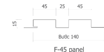
F-45 panel
