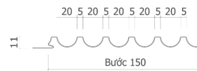
D-20 panel
