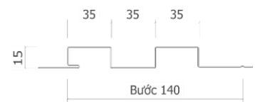
F-35 panel
