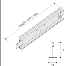
KHUNG T3660
