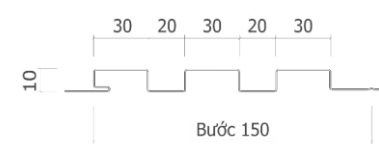
F-30 panel
