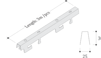
KHUNG F-SHAPED
