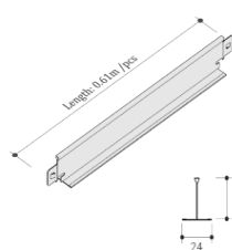
KHUNG T660
