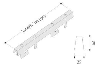
KHUNG F-SHAPED
