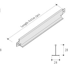
KHUNG T660
