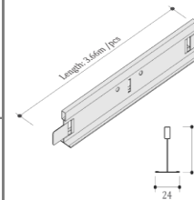
KHUNG T3660
