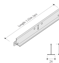
KHUNG T1220
