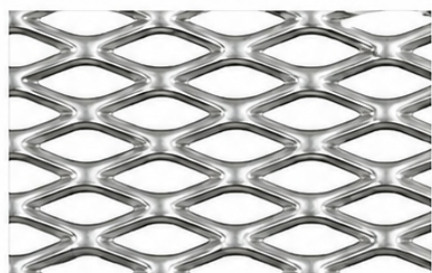
CLS5 Open area 42.5%, Thickness 2.5 mm Dimensions: 16 x 38 x 4.6 Weight 3.9 kg/m 2
