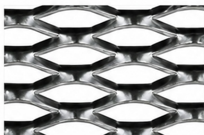
CLS7 Open area 69.4%, Thickness 2 mm Dimensions: 17 x 51 x 2.6 Weight 1.65 kg/m 2
