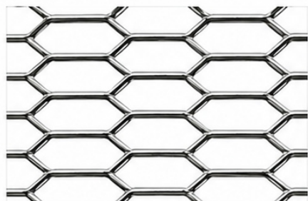
CLS1 Open area 69%, Thickness 2 mm Dimensions: 13 x 50 x 2 Weight 1.68 kg/m 2
