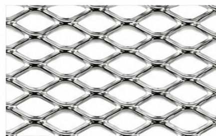
CLS12 Open area 52.7 %, Thickness 2 mm Dimensions: 11 x 25 x 2.6 Weight 2.56 kg/m 2
