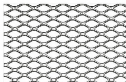
CLS3 Open area 42.5%, Thickness 2.0 mm Dimensions: 8 x 16 x 2.3 Weight 3.2 kg/m 2
