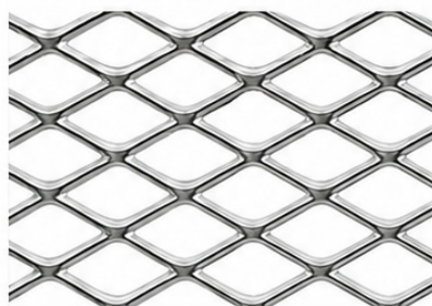
CLS2 Open area 66.7%, Thickness 2.2 mm Dimensions: 15 x 30 x 2.5 Weight 1.81 kg/m 2
